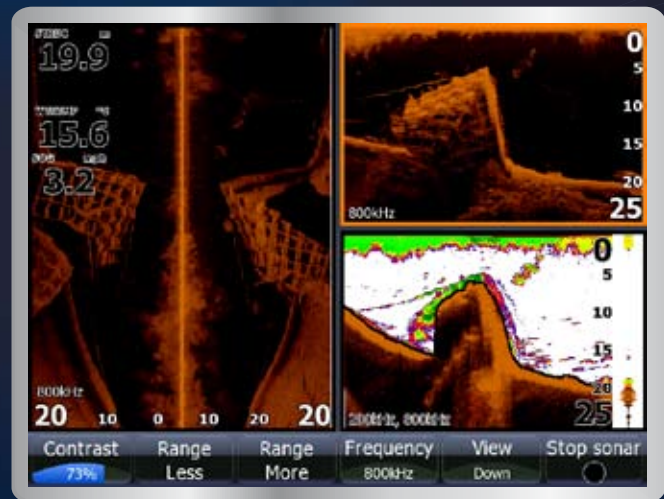
StructureScan - Get the whole picture: Combine all three technologies Broadband Sounder, SideScan, and DownScan™ into one all powerful angling tool.
